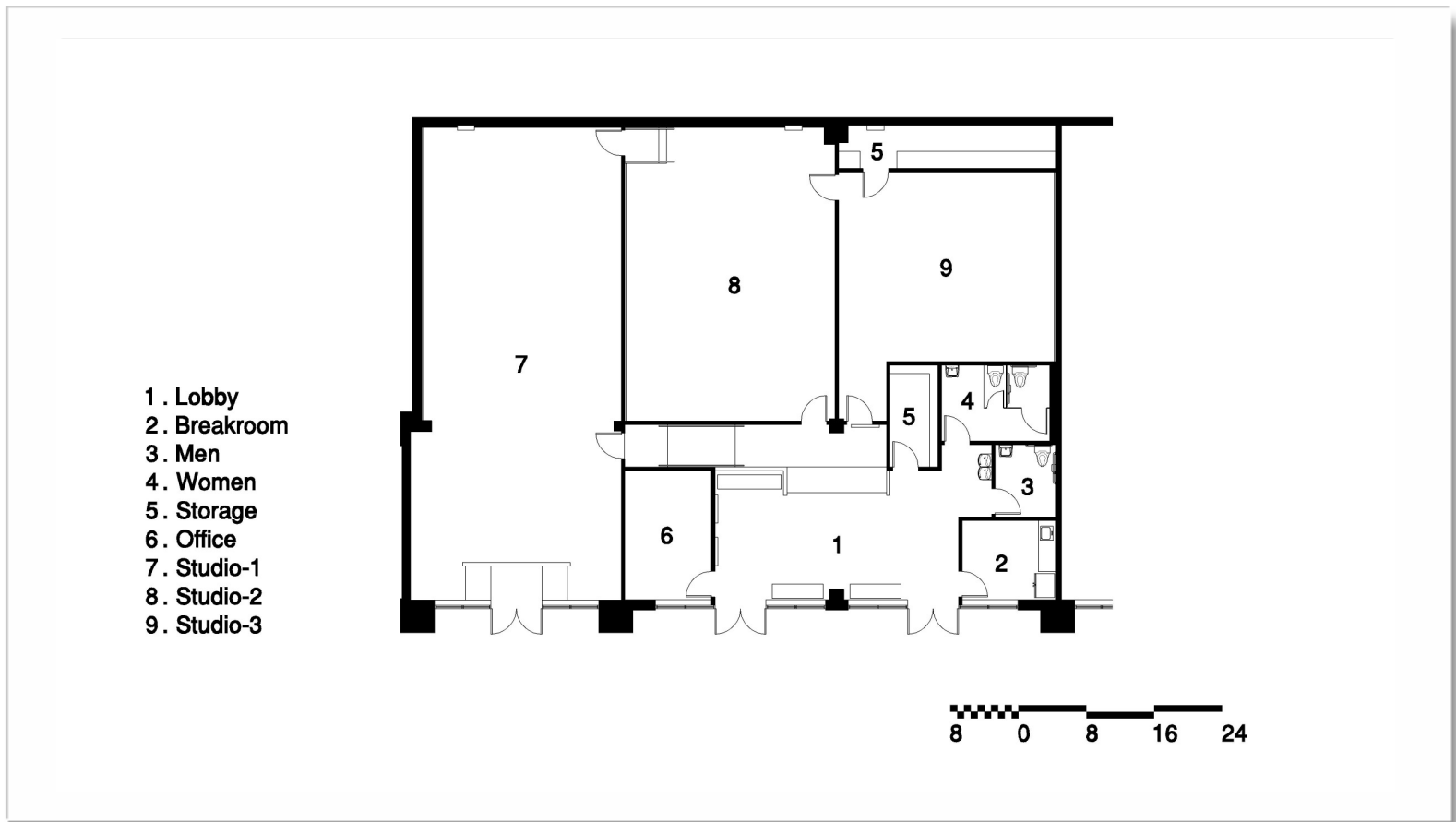
Plan View
